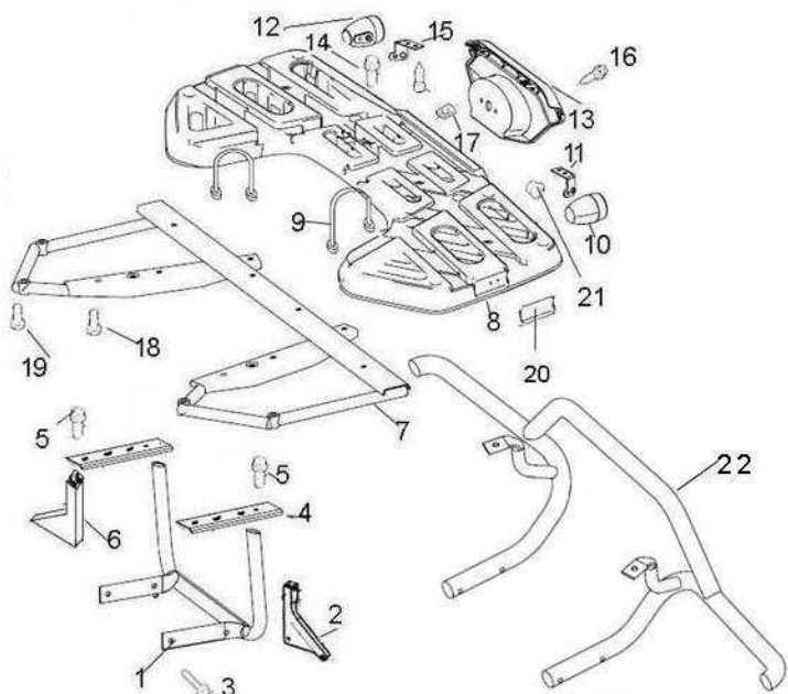
18 REAR RACK (FOR 50TH)
