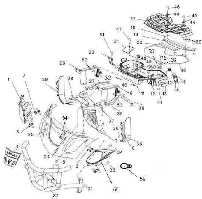
18 FRONT BUMPER & RACK ( FOR 50th )
