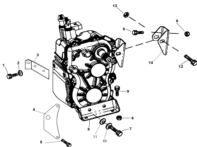
12 SUPPORT BRACKET
