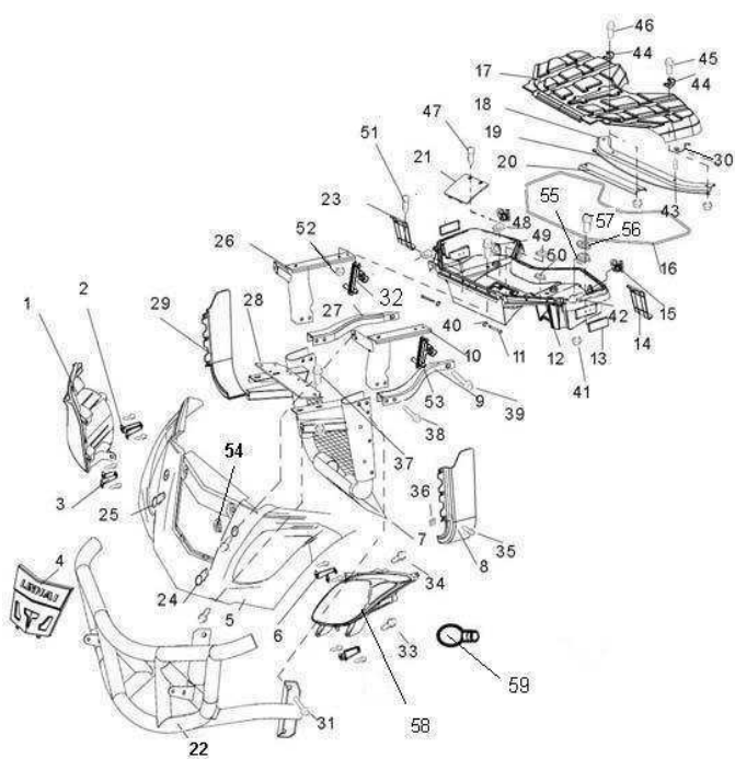
18 FRONT BUMPER & RACK ( FOR 50th )
