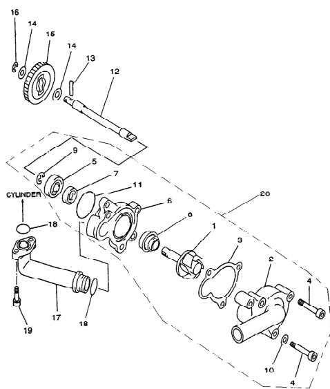
23 WATER PUMP
