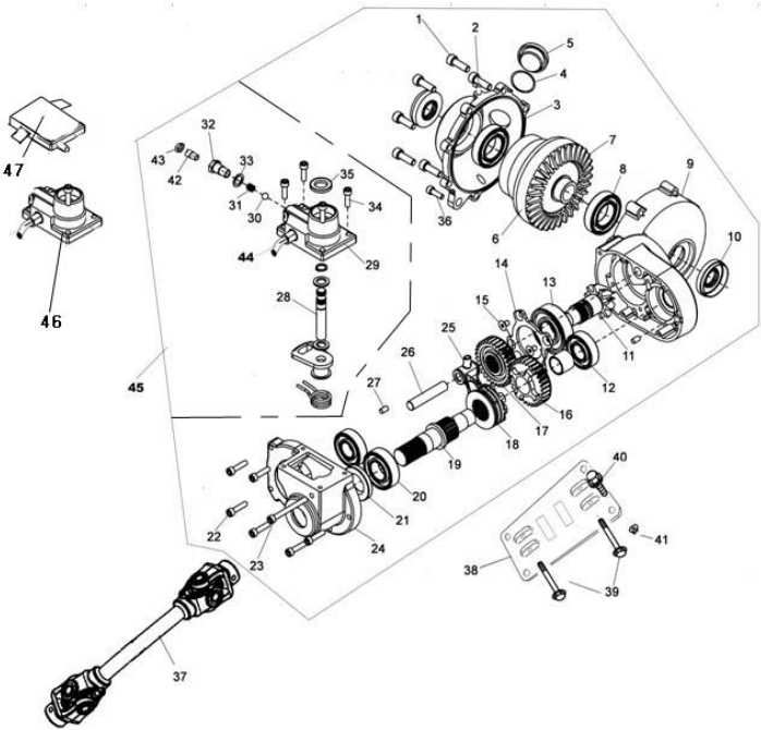
36 FRONT GEAR-BOX ( FOR 4WD )
