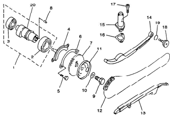
22 CAMSHAFT CHAIN
