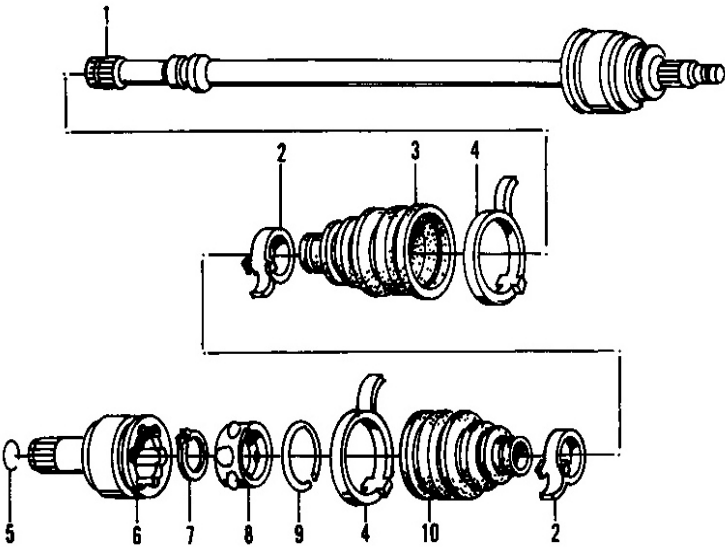
37 FRONT DRIVE AXLE ( FOR 4WD )
