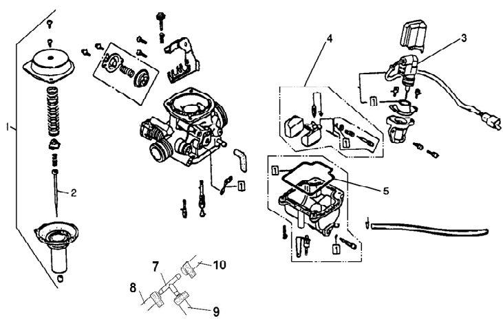
27 CARBURETOR
