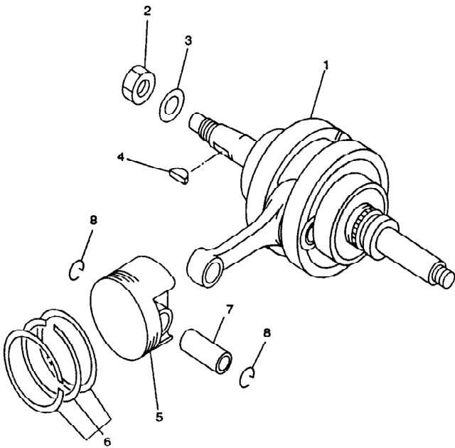
20 CRANKSHAFT COMP
