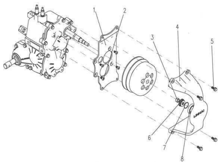
HIGH-POWER CLUTCH STAND ASSY
