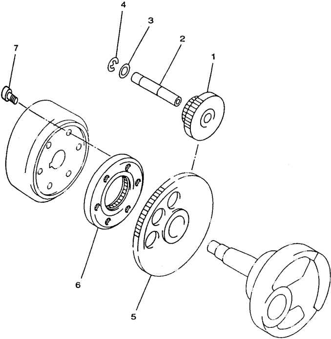
31 STARTER
