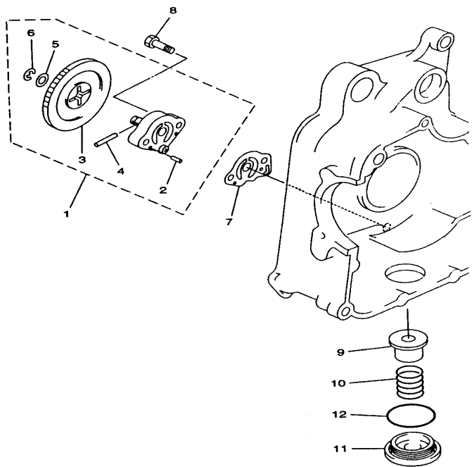
25 OIL PUMP
